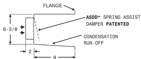
RH SIDE VIEW
