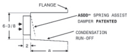
RH SIDE VIEW
